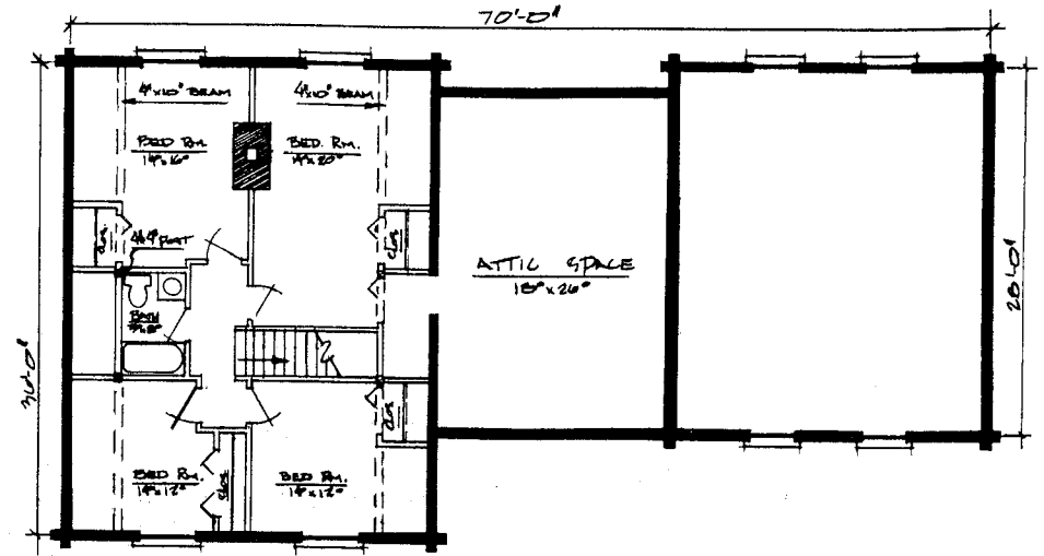
SECOND FLR PLAN
