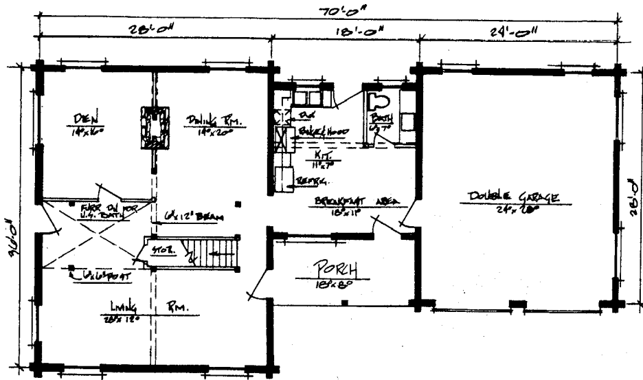
FIRST FLR PLAN
